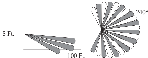
Figure 2 - Coverage Angles
